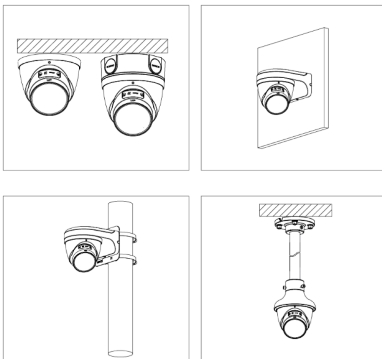
Figure 3-3 Installation method
