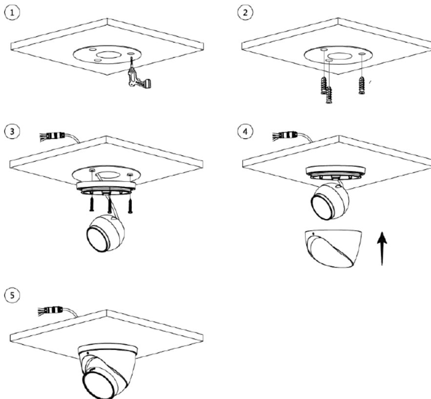
Figure 3-6 Cable going through the mounting surface
