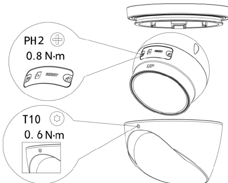
Figure 3-4 Detach the enclosure
