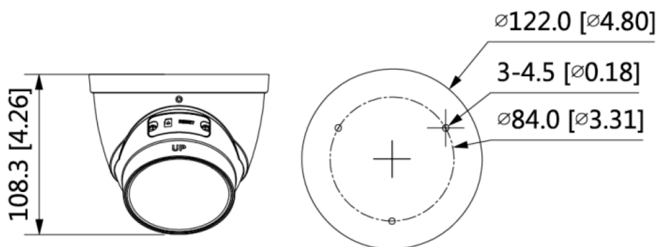
Figure 3-2 Dimensions (Unit: mm [inch])
