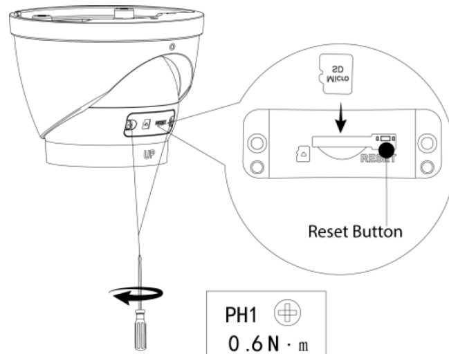
Figure 3-5 Install SD card
